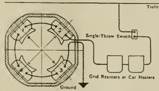
FIG. 1. CONNECTIONS FOR MAKING TEST ON MAIN COILS.
